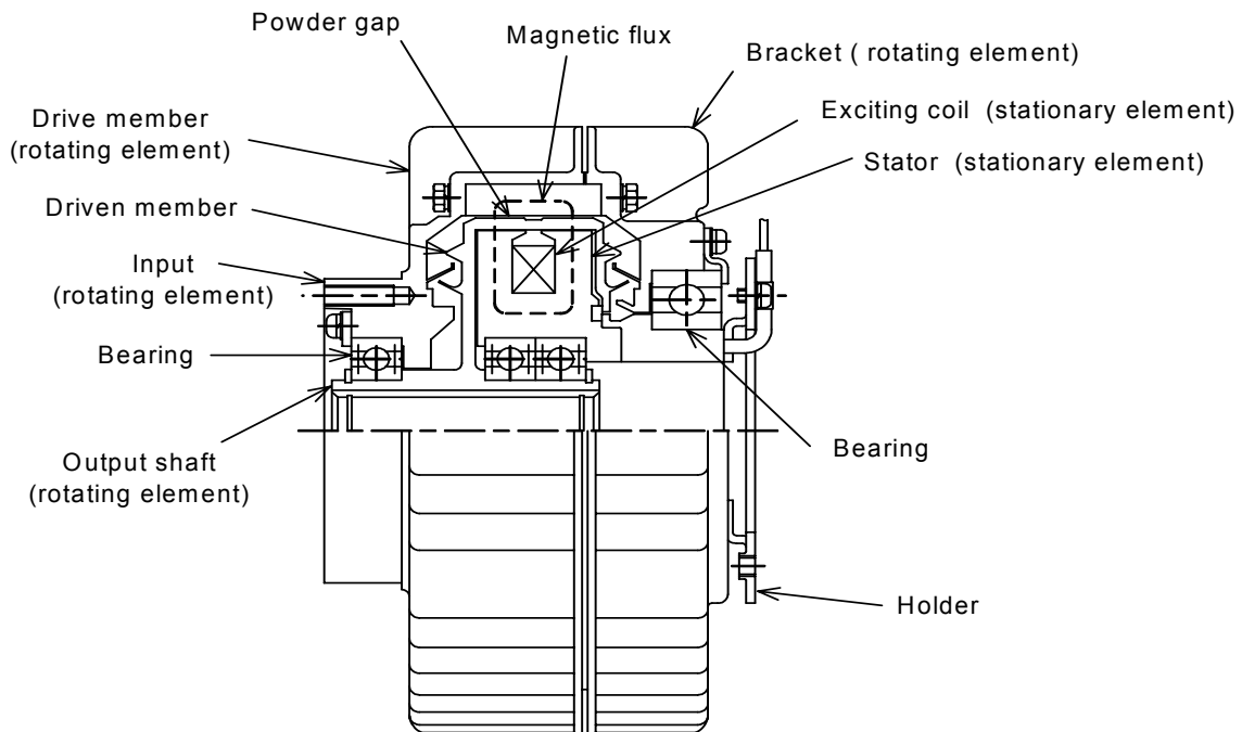
Fig. 1 Structural diagrams of ZA-AN 1 powder clutches (representative examples)
