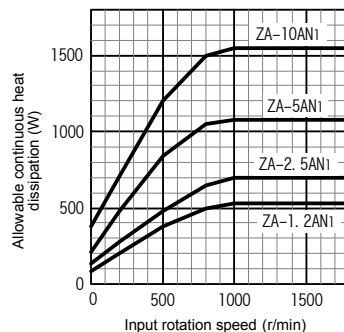
Fig. 3 Allowable heat dissipation characteristics
